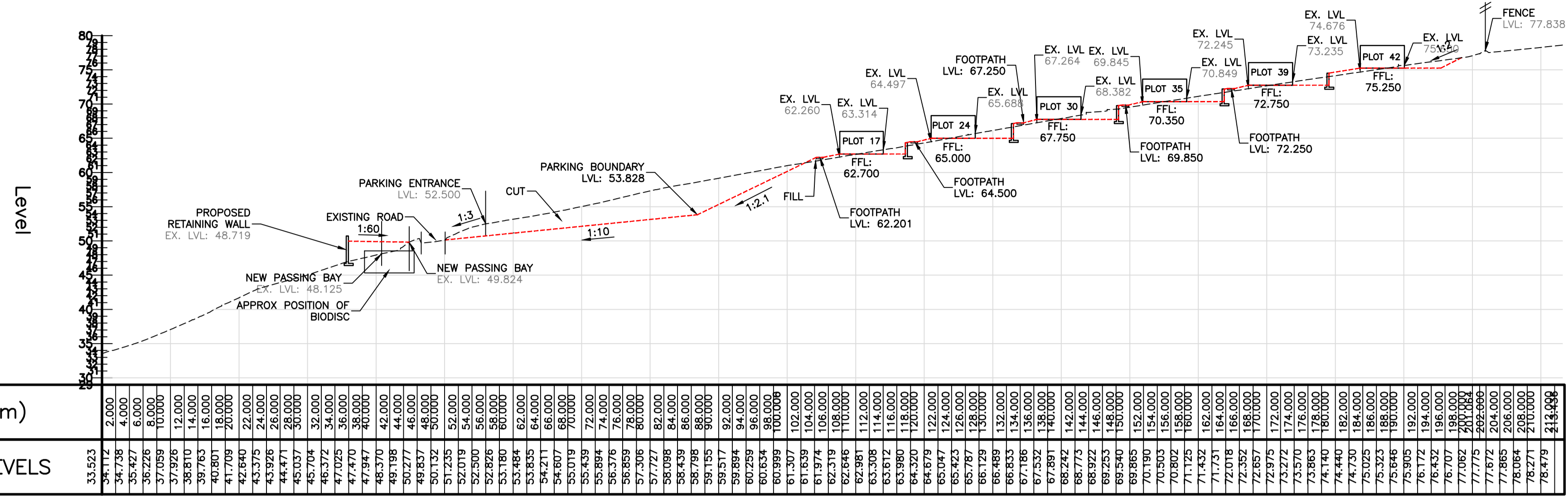
SITE SECTION – EXISTING AND PROPOSED SURFACE 1:500
