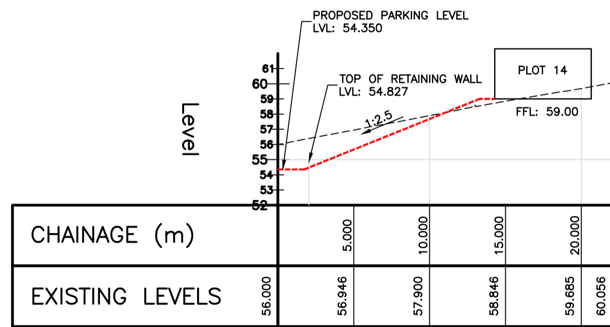
SECTION 2-2 1:250
