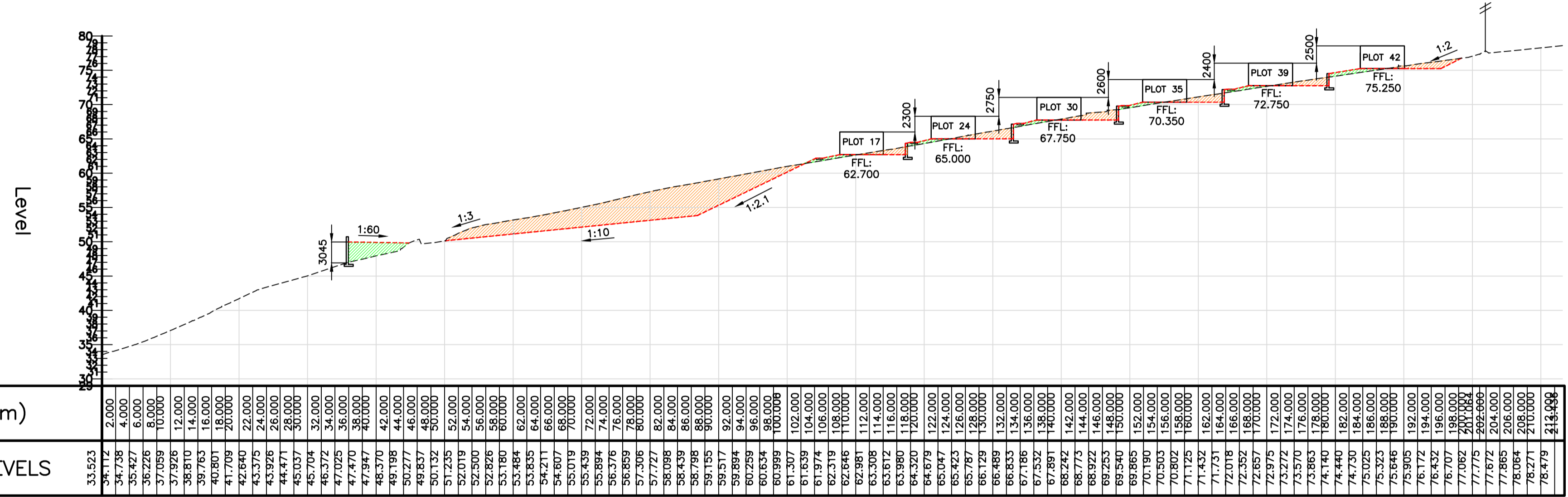
SITE SECTION – CUT AND FILL 1:500
